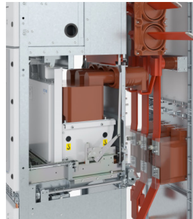
Current and voltage transformers located in the bus riser.
