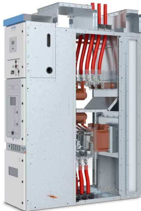
Single width panel solution with cable in/out (top/bottom).
